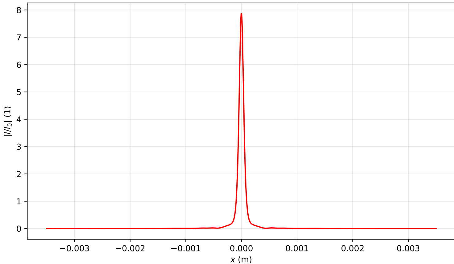
Intensity profile I(x, y = 0, z = 3.662)/I_0 , P_{in}=4.0P_{cr} , artificial time
